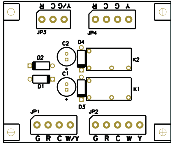
Main Board
